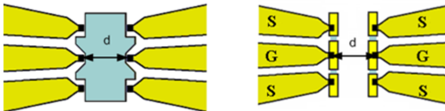
Figure 3. Probe spacing
