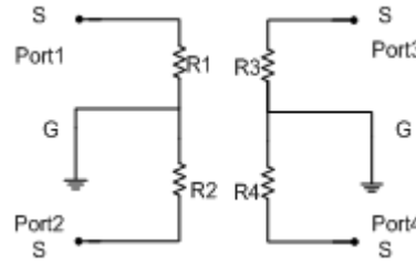
Figure 7. Electrical model
