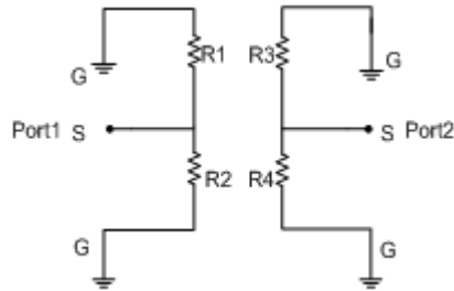
Figure 7. Electrical model
