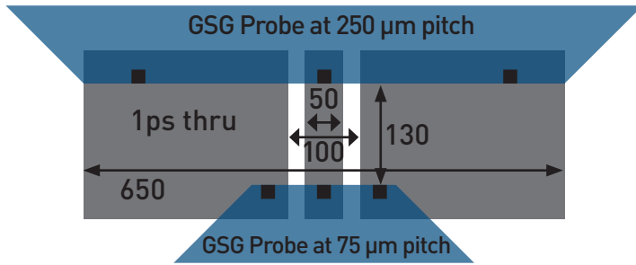
Figure 2. Dimensions of the 1 ps thru standard in ISS P/N 101-190 (units in \mu\text{m} ).
