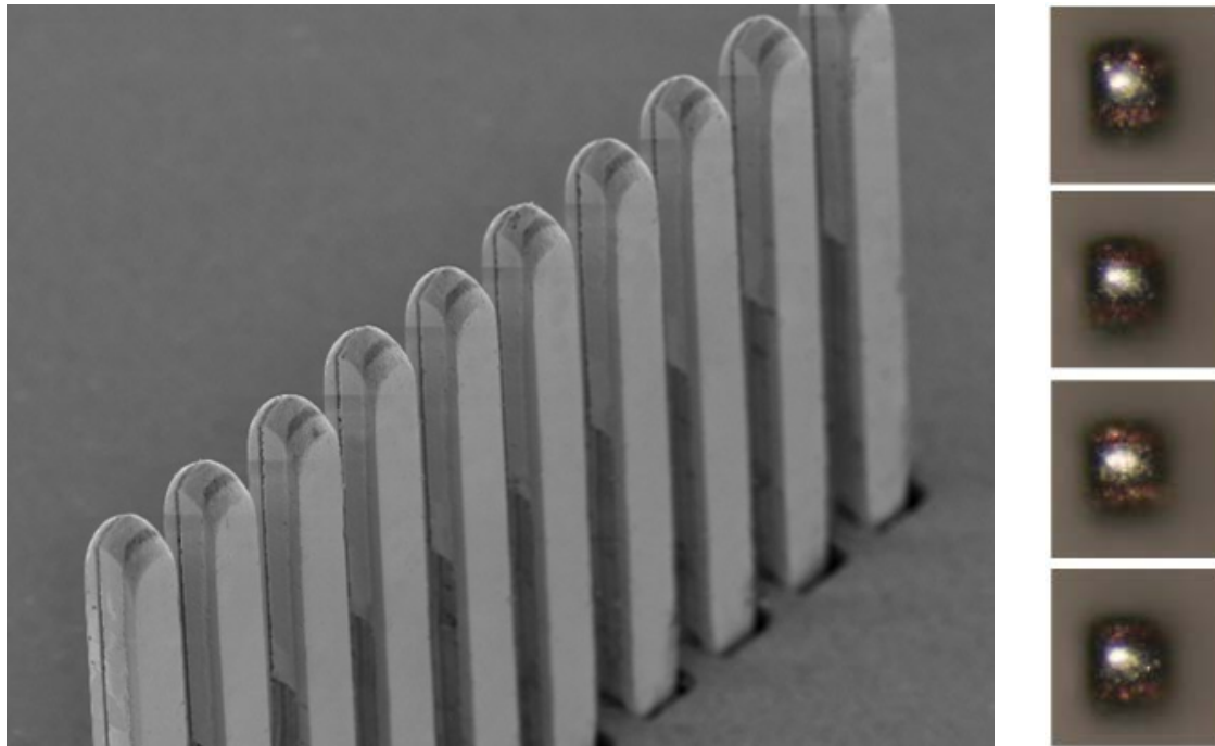
60um pitch SEM and Optical Images
