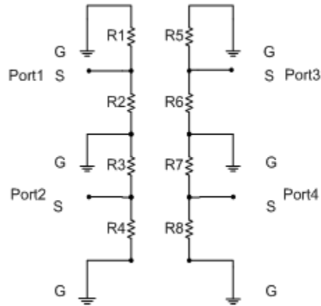
Figure 7. Electrical model
