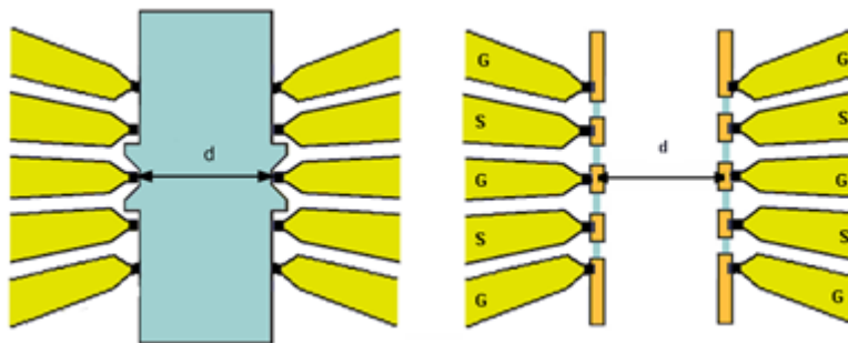
Figure 3. Probe spacing
