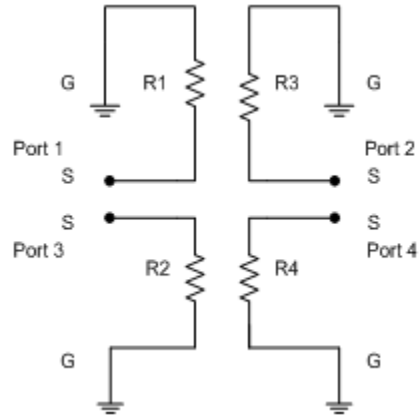
Figure 7. Electrical model
