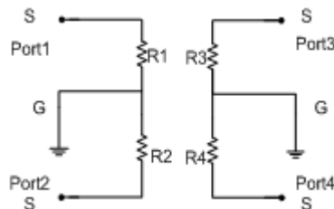
Figure 7. Electrical model
