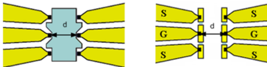
Figure 3. Probe spacing
