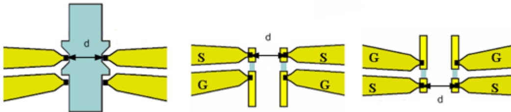
Figure 3. Probe spacing
